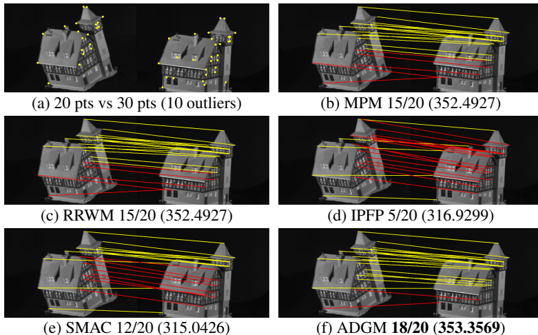
Figure 1: House matching using the pairwise model B described in Section 4.1. Ground-truth value is 343.1515. (Best viewed in color.)
