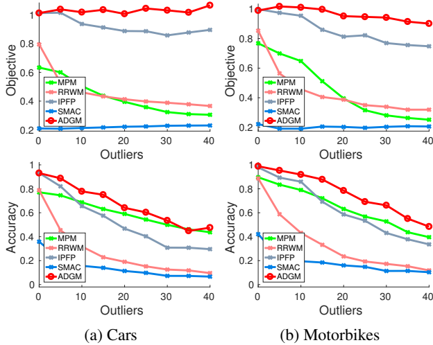
Figure 4: Results on Cars and Motorbikes using the pairwise model C described in Section 4.2.
